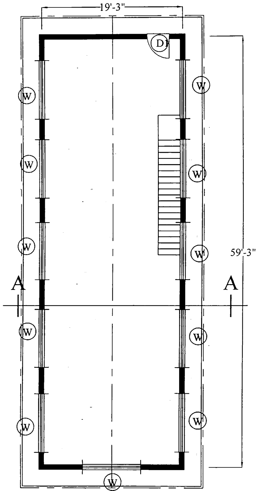
UPPER PLAN
